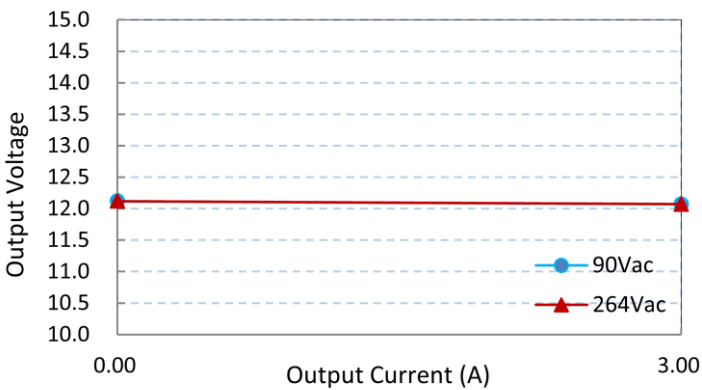
Load Regulation (12V/3A)
