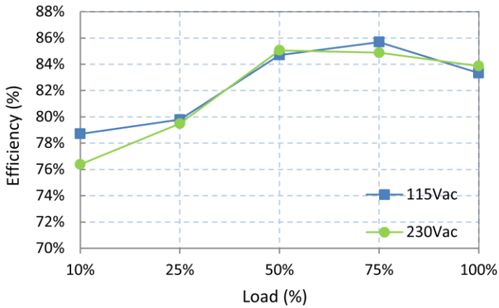
Efficiency (20V/2.25A)
